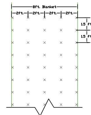
Figure D - Plan View
